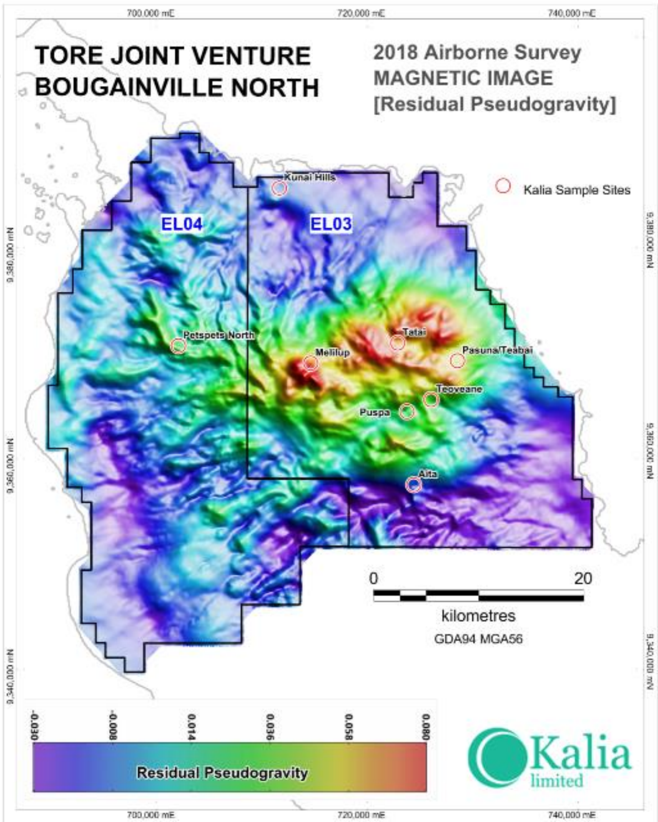
Figure 1 - Residual Pseudo-gravity data (Preliminary Image)
